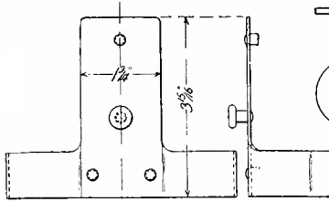
BEARING-THICKNESS GAUGE 3 3/4 x 7 & 4 1/2 x 8 JOURNALS
